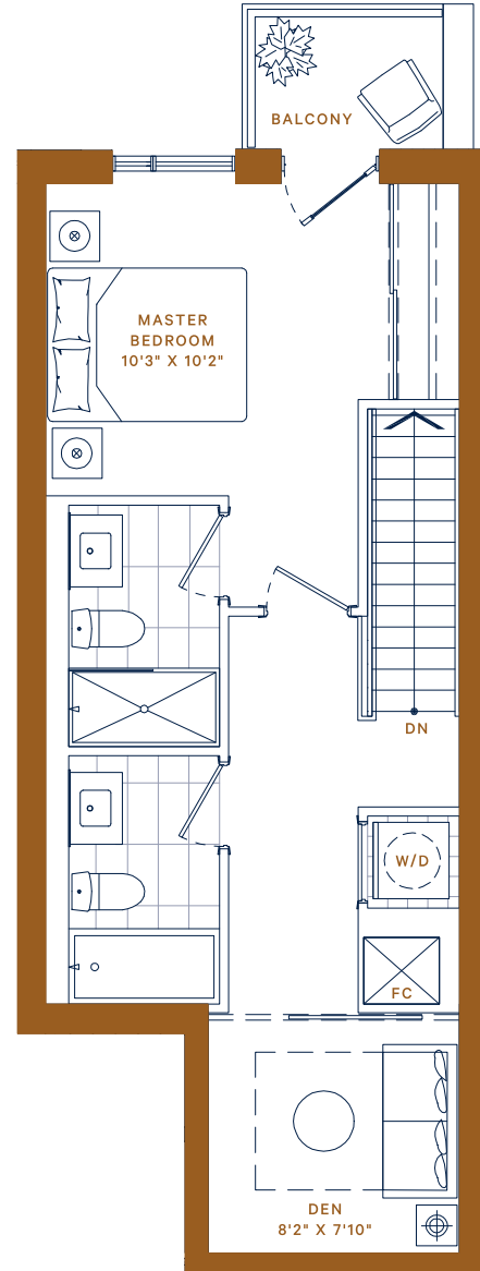
UPPER LEVEL
